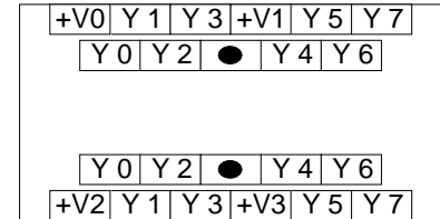
Figure: 2.15 FX0N-16EYT-ESS/UL
