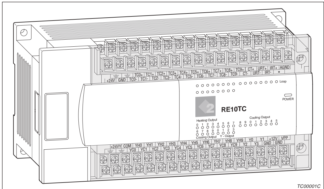
Fig. 1-1: Temperature Control Module FX2N-RE10TC
