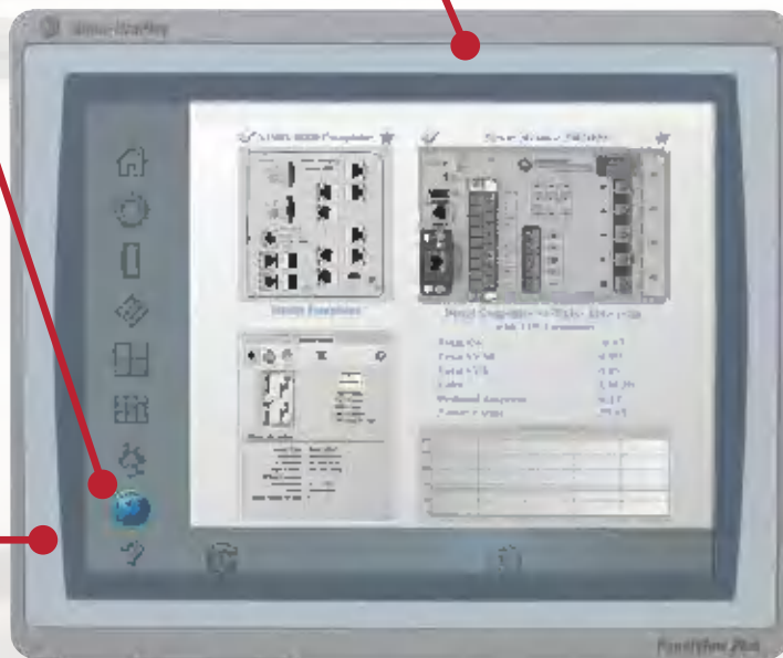
STANDARD MODEL
