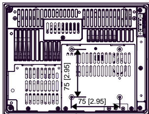
PS-3451A not built-in HDD unit
